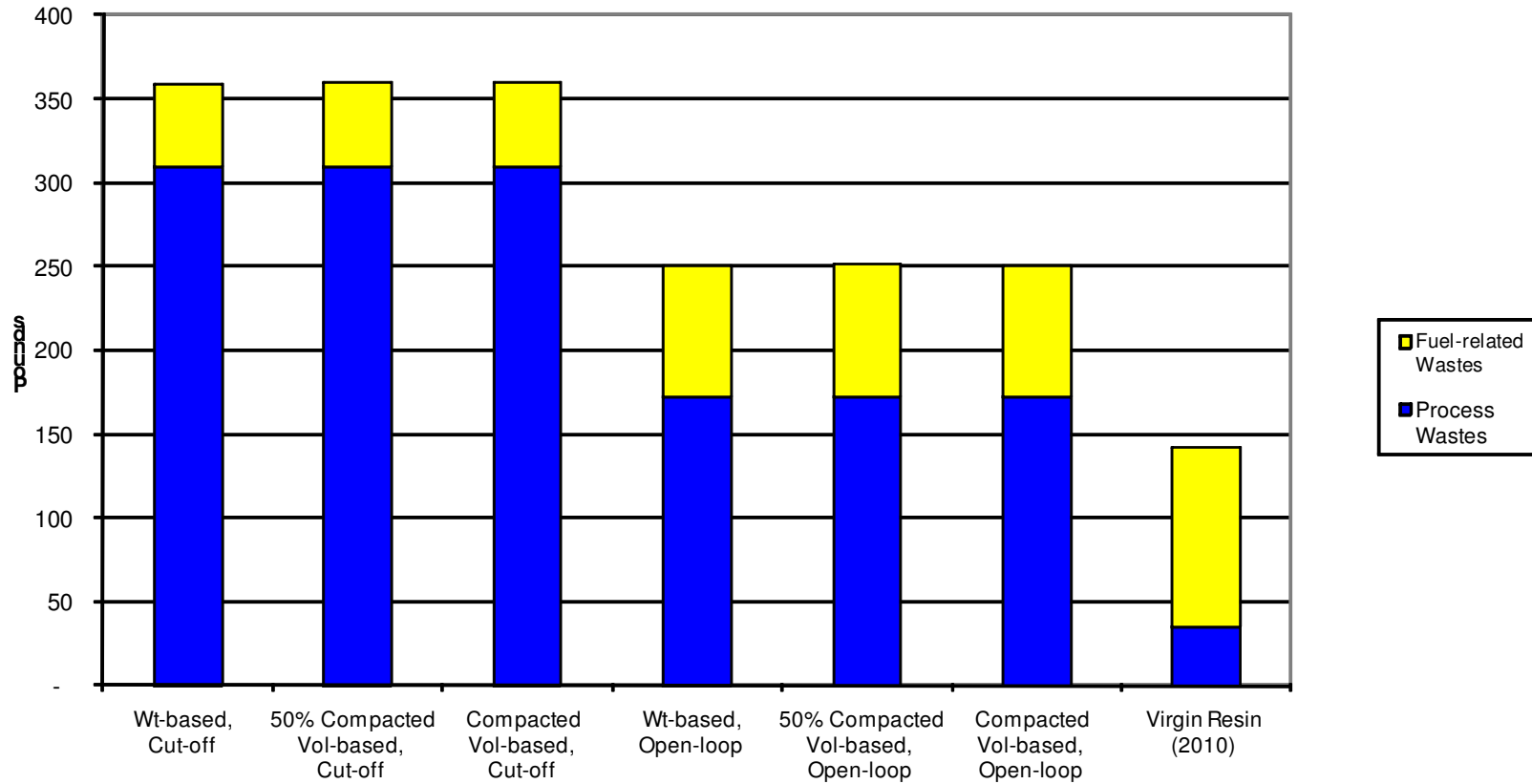
Figure 3-3b. Solid Waste Results by Solid Waste Category for Production of Recycled PET Resin Flake (pounds per 1,000 pounds of resin)
